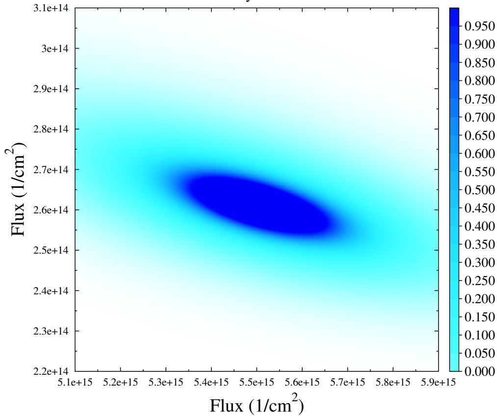
Probability distribution
