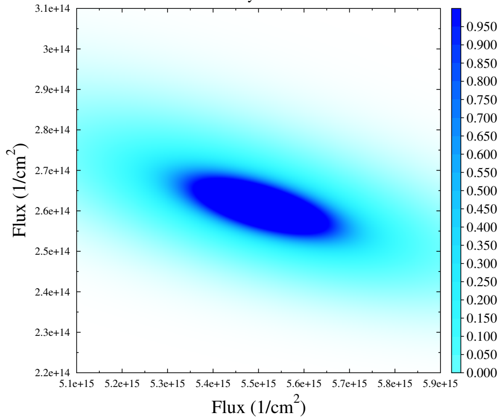
Probability distribution
